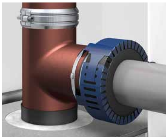
Curaflam® Konfix Pro – firestop from mixed installations
